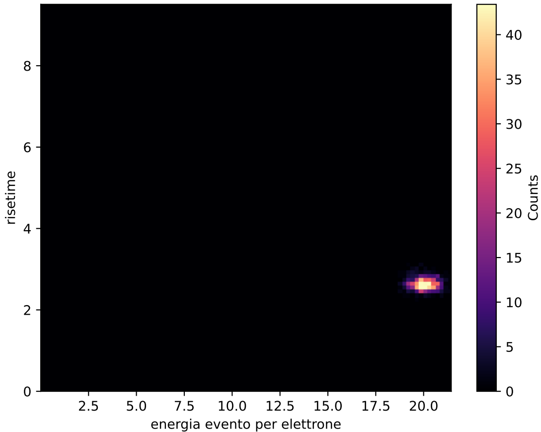
electron distribution 20.0GeV
