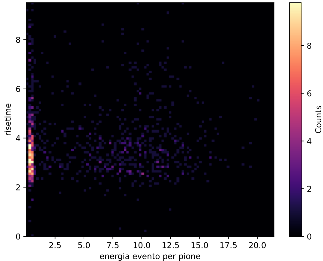
pion distribution 20.0GeV
